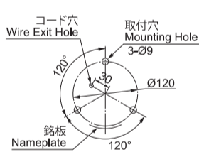
取付面寸法図 Installation Dimensions
